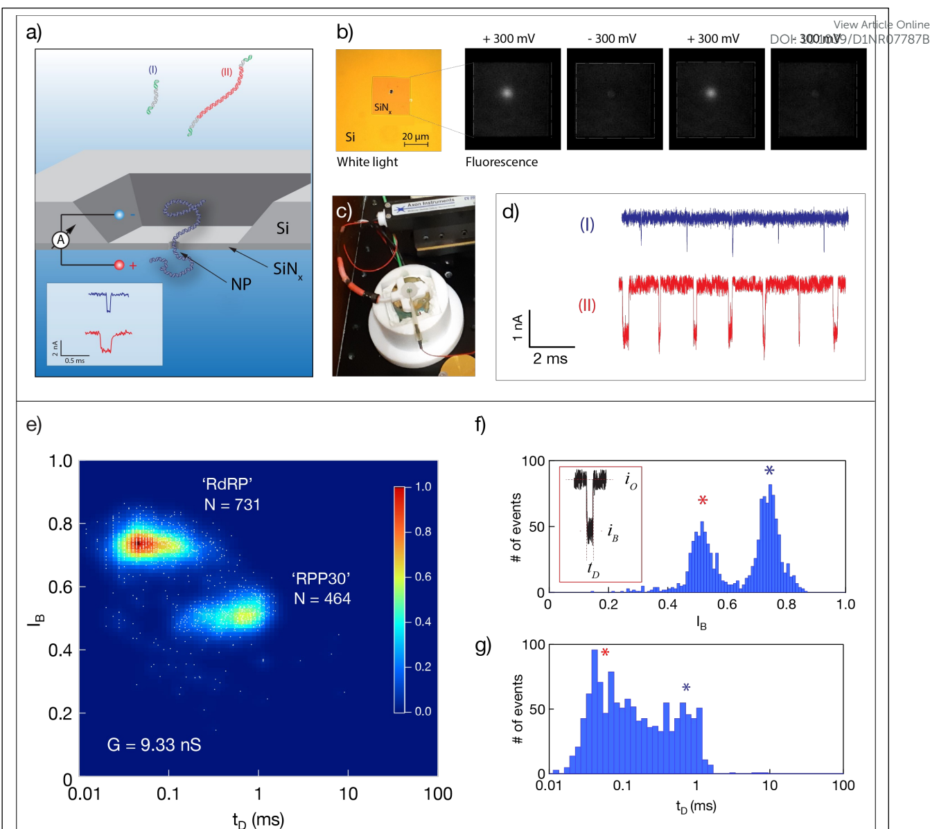
Fig 1 Solid-state nanopore-based sensing of SARS-CoV-2 RNA validation using synthetic RNA samples. a. Schematic illustration of the method. RNA molecules corresponding to the two target genes (I and II) are first reverse transcribed. The resulting dsDNA molecules are then sensed using a ssNP. The dsDNA strands of the two target genes are designed to be 107 bp and 758 bp, respectively, enabling single molecule counting using a \sim 5 nm ssNP. b ssNPs are fabricated in a 25 \mu\text{m} square silicon nitride membrane. Wide-field fluorescence image of a typical ssNP using under \pm 300 mV and calcium indicator dye, RHOD-2. c. The measurement apparatus consists of two small fluidic chambers, filled with an electrolyte solution and connected by Ag/AgCl wire electrodes to a current amplifier. d Typical ion-current blockade events associated with RPP30 dsDNA (human reference gene, blue) and RdRP dsDNA (viral gene, red). e. A characteristic event density diagram for the two genes produced from synthetic RNA sources and analysed separately using the same ssNP ( G = 9.33 nS). The two distinct event populations are distinguished by (f) their fractional blockade level ( I_B ) and (g) typical event dwell times ( t_D ).
