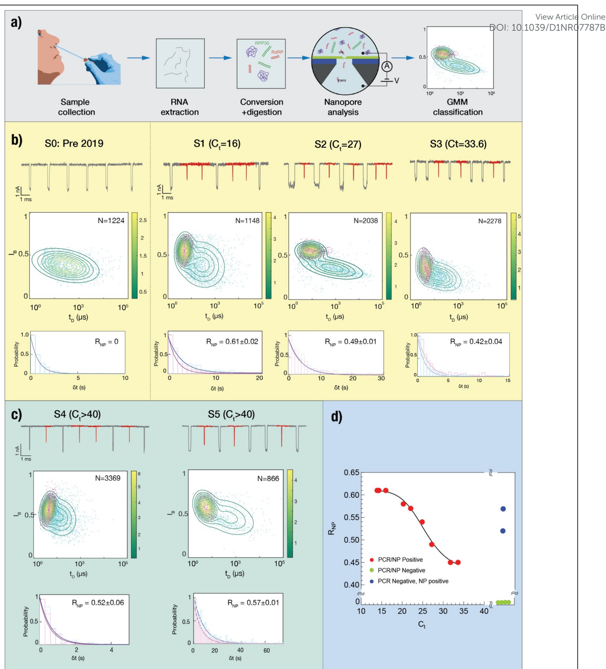
Fig 2 Single molecule analysis of clinical SARS-Cov-2 samples. a) A general flow of the sample treatment and ssNP-based sensing for clinical samples. Nasal swabs collected using standard protocols are immediately suspended in virus-inactivated lysis buffer, followed by RNA extraction (on site). RNA to DNA conversion is done in a single step using specific oligonucleotide primers for the target genes, as well as RT and DNA polymerase for second strand synthesis. Then all single stranded nucleic acids and proteins are enzymatically digested, and the sample is analyzed using an ssNP of roughly 4 nm diameter. The dsDNA translocation events are clustered in two groups representing the abundance of the two target genes in sample using GMM. b) Four clinical samples with increasing C_t value, analysed consecutively using ssNPs with an average conductance of 13.8 \pm 1 nS. S0 is Pre-Covid-19 sample, used as a true negative control. Upper panels: typical events traces in which the events assigned to RdRP gene fragments are marked in red, and the events assigned to RPP30 are in grey. Middle panels: The two distinct populations of the SARS-CoV-2 RdRP gene (magenta) and human reference gene RPP30 are classified using a two-dimensional GMM algorithm. Lower panels: the annotated translocation events are used to calculate the event rate for each gene, from which the SARS-CoV-2 ratiometric nanopore index is calculated. c) Analysis of two SARS-Cov-2 clinical samples for which RT-qPCR results were classified as negative. In both cases the nanopore index is moderate, suggesting that these samples are likely false negatives. d) Comparison of ssNP analysis and RT-qPCR for nine clinical COVID-19 samples. The data set of positive samples (red points) is empirically fit using a non-linear Hill function (solid line). Green points represent samples that were negative (undetermined) in RT-qPCR as well as in the nanopore analysis. Blue points represent samples that were found negative (undetermined) by RT-qPCR, but positive in the nanopore analysis. The expected C_t values of these samples are estimated by the non-linear Hill function.
